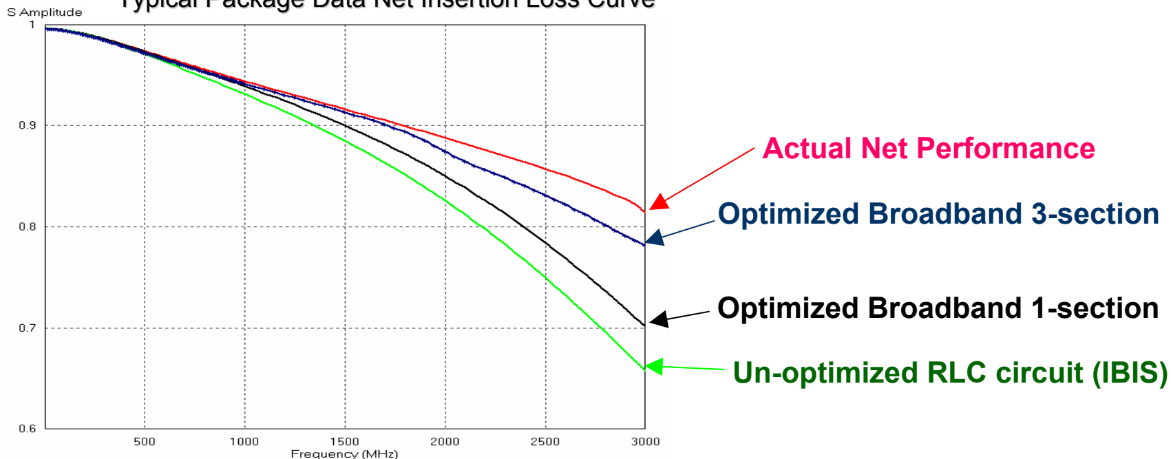
Typical Package Data Net Insertion Loss Curve
