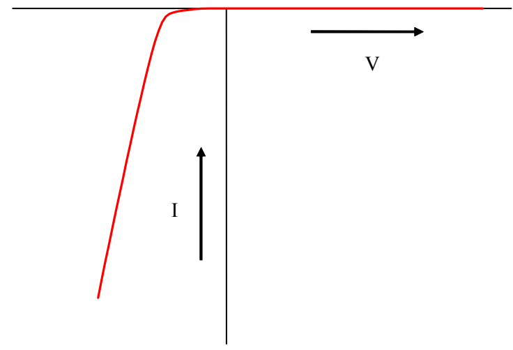
Figure 5.4 – Graph of [GND Clamp] I-V Table Data
