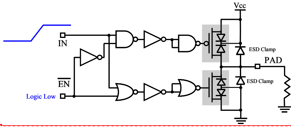
Figure 3.2 – Simulation Setup for Extracting Ramp Rate Information (Rising Edge Shown)
