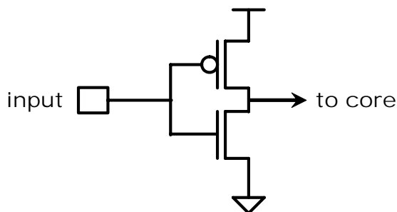
Figure 4.4 – Single-ended Receiver
