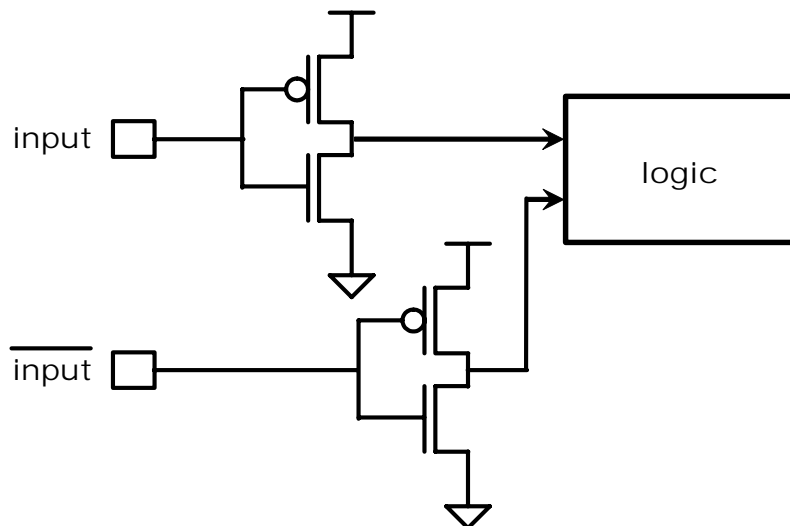
Figure 4.7 – Pseudo-differential Receiver
